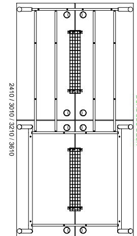
4 SEATER 4-WAY DUAL SETUP
